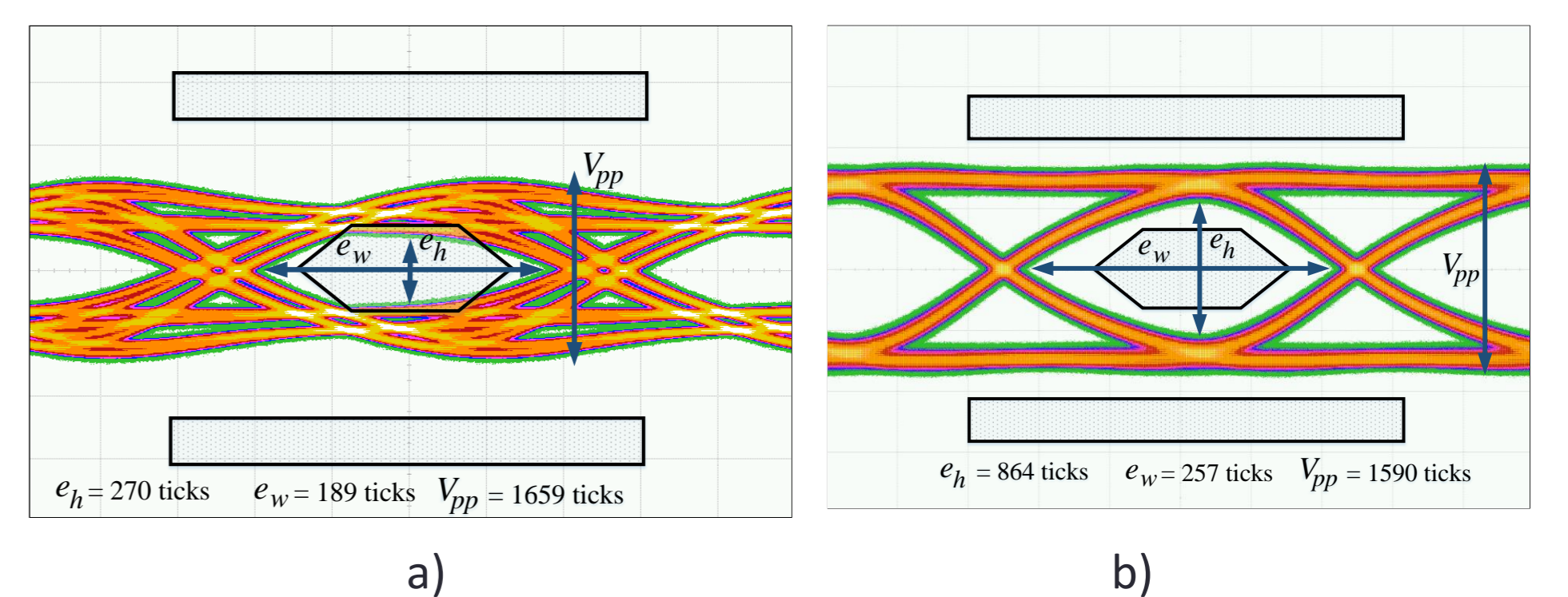
Fig. 4.2. Eye diagram over mask: a) before optimization; b) after optimization.
