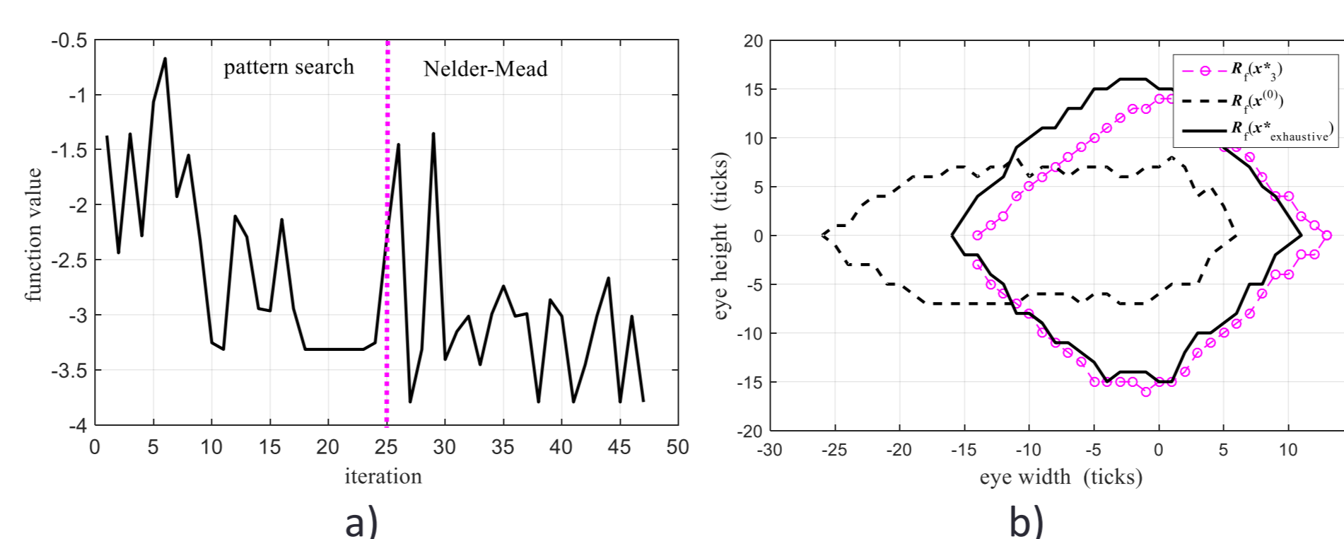
Fig. 3.3. a) Objective function across iterations; b) Eye diagram: proposed methodology ( R_i(x^*) ) vs initial design ( R_i(x^0) ) vs current method ( R_i(x^* \text{ exhaustive}) ).
